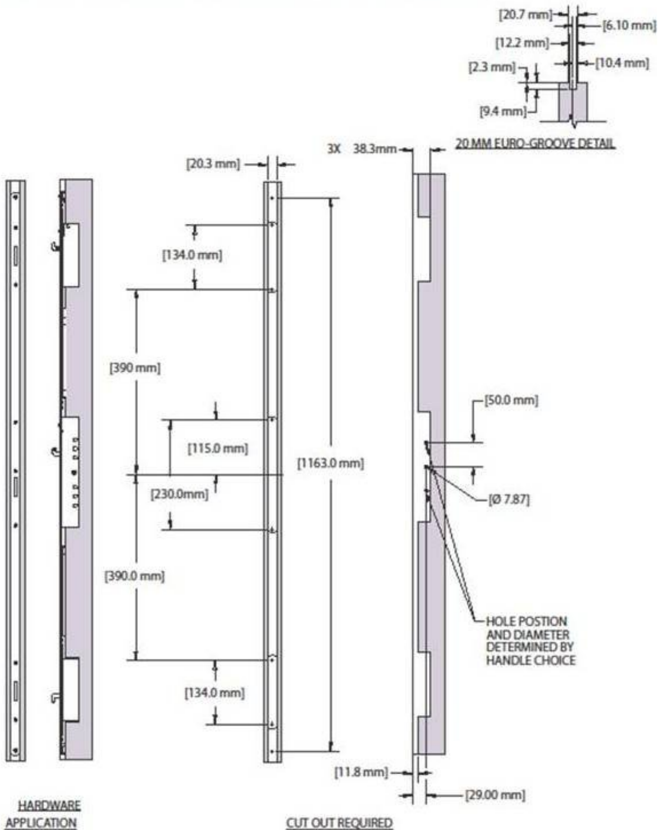
FIG. 15 THREE POINT MORTISE LOCK, 20mm EURO-GROOVE APPLICATION
